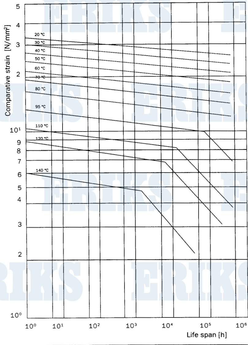
Creep resistance of SIMONA® PVDF
