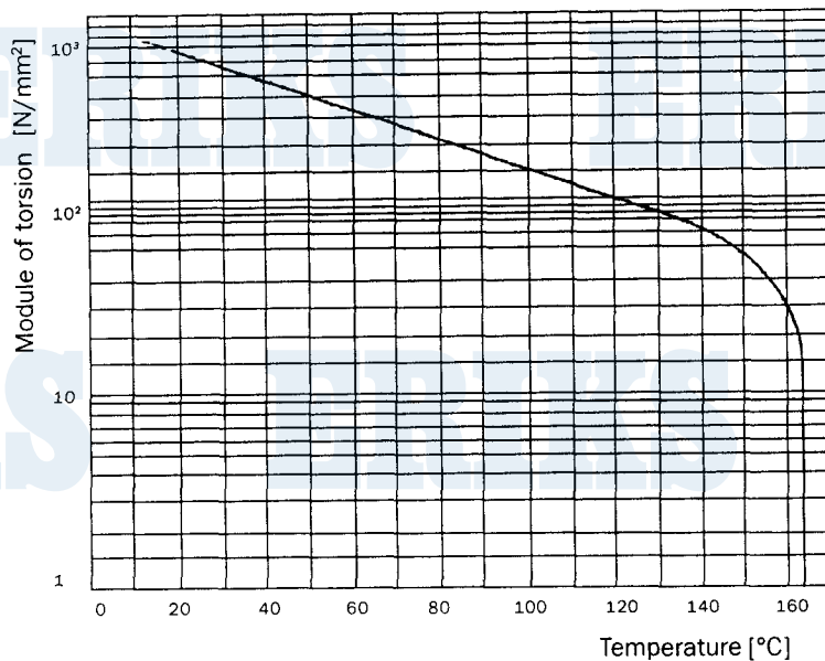
Module of torsion of SIMONA® PVDF
